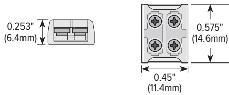
ESTLK-60: 60" Tape-to-Tape
