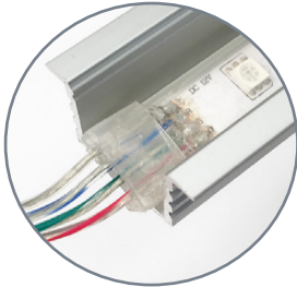
LED-CHL-XD-F channel is perfect for wet location and RGB tapes
