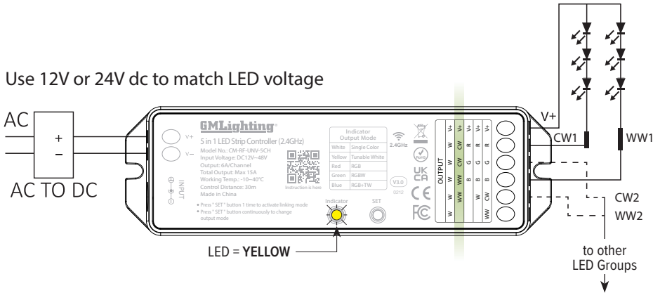
CM-RF-UNV-5CH RF Controller
