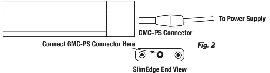
SlimEdge End View
