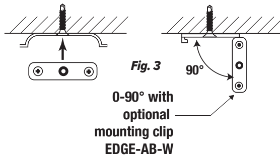
SlimEdge End View
